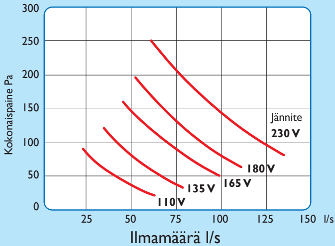
AirWay Motor 160 mm
